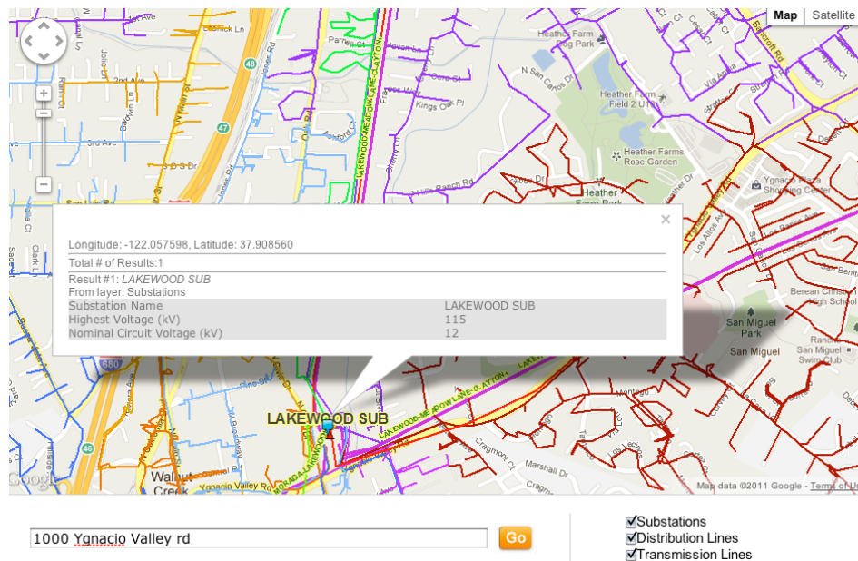
Figure 1: Distribution Grid Interconnection Map vii
