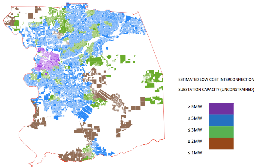
Figure 1: SMUD Distribution Grid Interconnection Map iv
